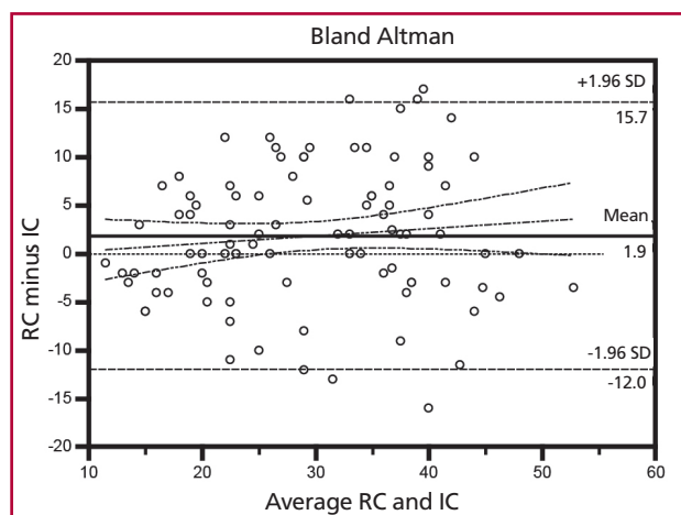
Fig. 1. Classic Bland-Altman plot.
