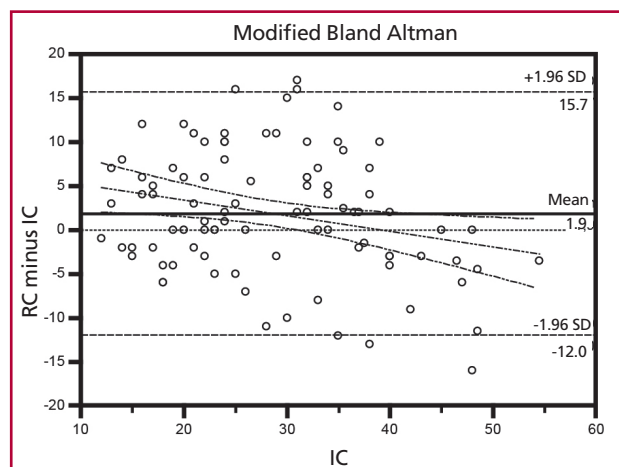
Fig. 2. Modified Bland-Altman plot according to the reference method.
